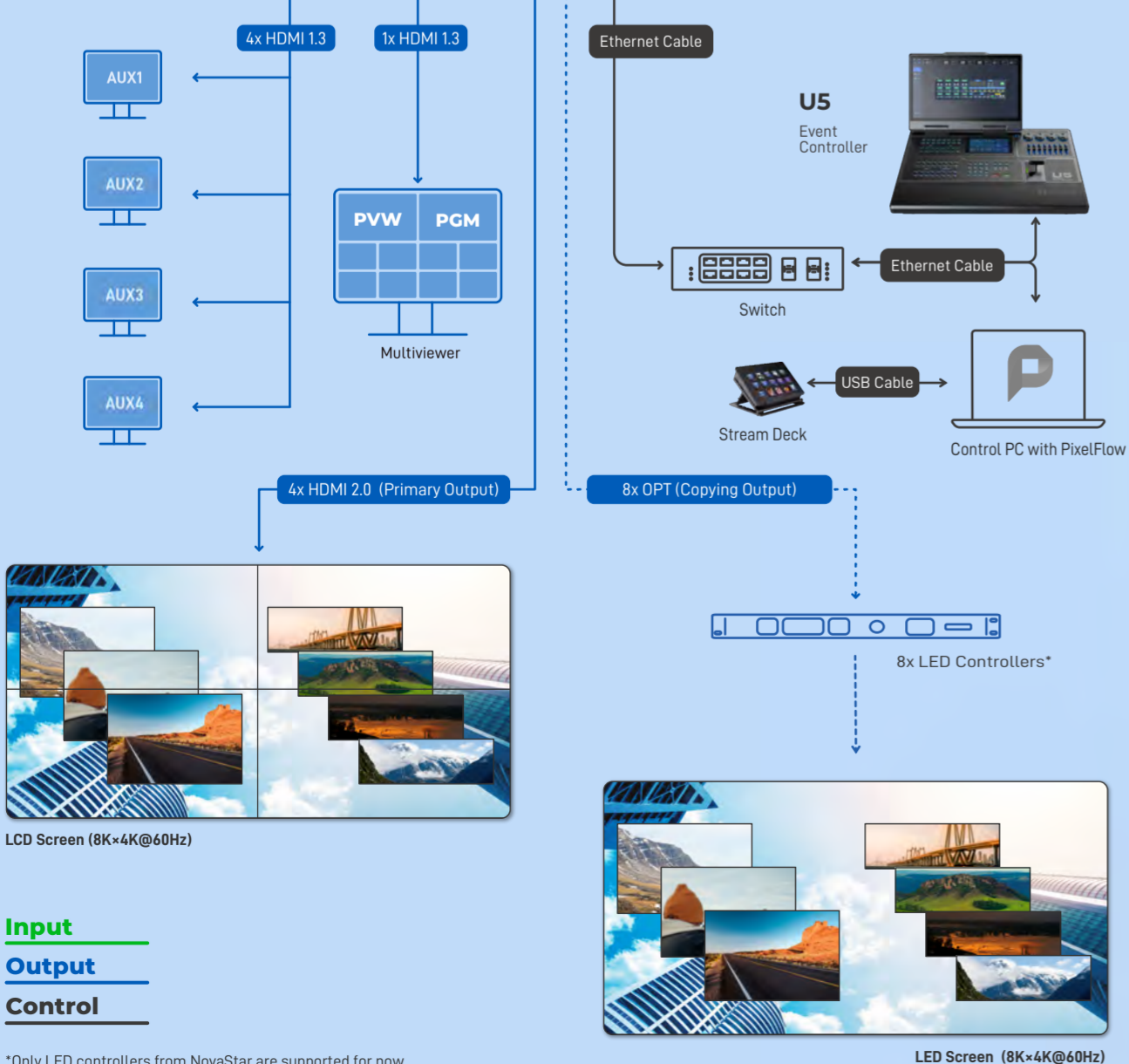
LED Screen (8K*4K@60Hz)
